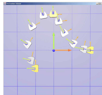
Figure 2: Design positions
