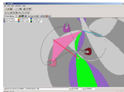
Figure 13: Solution Map for 3-position option
