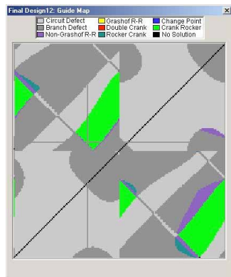
Figure 3: Solution map
