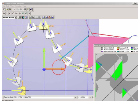
Figure 4: Solution to design positions
