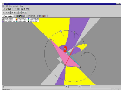
Figure 1: 3pt motion solution map
