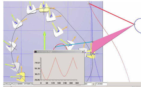
Figure 11: Alternative solution with better transmission angle
