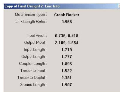
Figure 7: Linkage information
