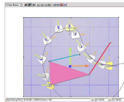
Figure 12: 3-position motion generation
